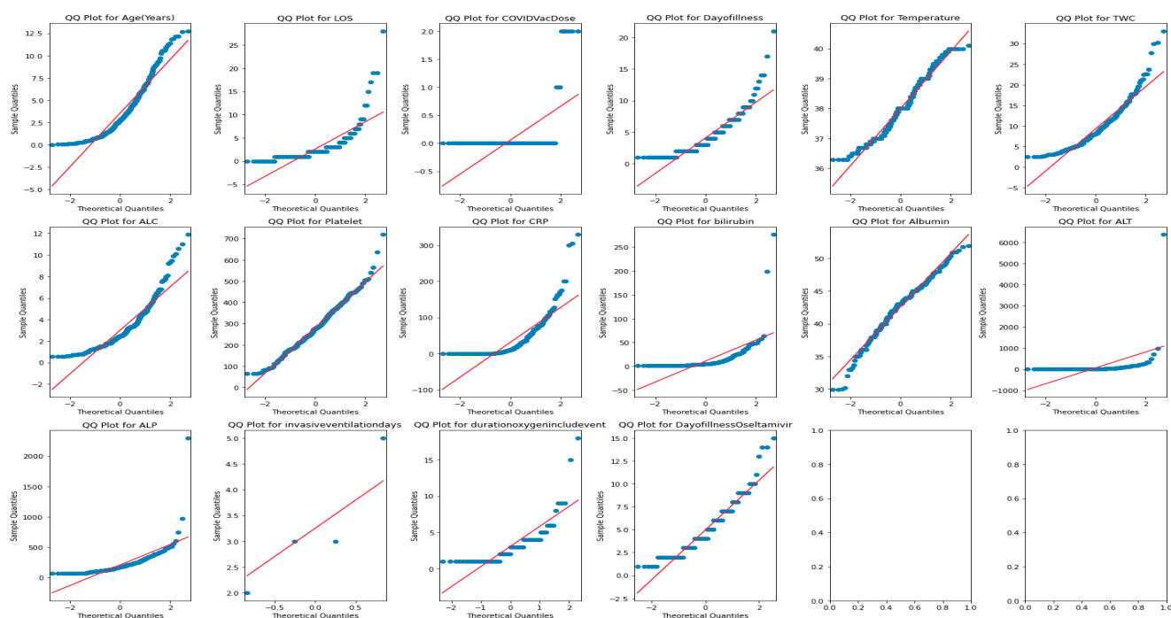
Supplementary Fig. 1. Quantile-quantile plots for continuous variables. This figure shows QQ plots for the continuous variables. The red diagonal line represents the theoretical normal distribution reference line under normality. Deviations from this line indicate skewed from normality. All QQ plots displayed nonlinear patterns, indicating that all tested continuous variables deviated from a normal distribution. LOS, length of stay; TWC, total white cell; ALC, absolute lymphocyte count; CRP, C-reactive protein; ALT, alanine aminotransferase; ALP, alkaline phosphatase
