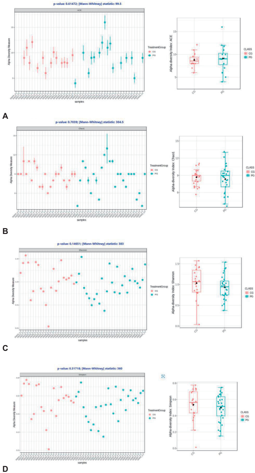
Supplementary Fig. 4. Alpha diversity at V2 (35 weeks' postmenstrual age). (A) Abundance-based coverage estimator (ACE) index. (B) Chao1 index. (C) Shannon index. (D) Simpson index. No significant intergroup differences were noted in any parameters.
