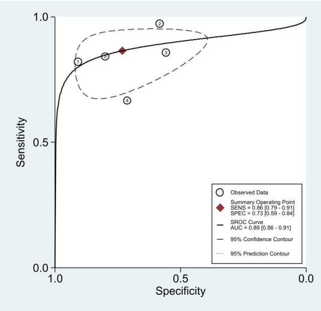
Supplementary Fig. 5. Summary receiver operating curve with confidence and prediction regions. Sens, Sensitivity; Spec, Specificity; SROC, Summary Receiver Operating Characteristic; AUC, Area Under the Curve
