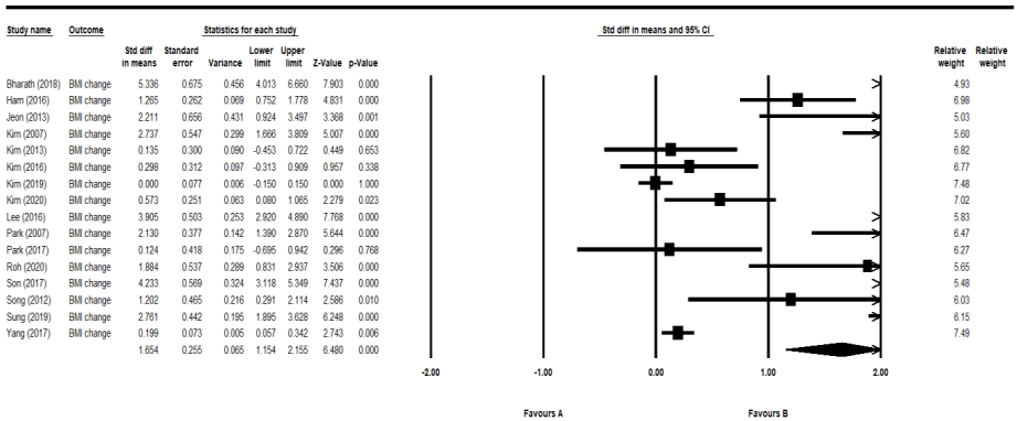
Supplementary Fig. 3. Forest plot after removing three studies: Cha (2019), Cha (2020), and Kim (2010).
