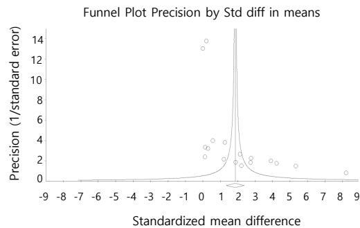
Supplementary Fig. 2. Funnel plot after removing 2 studies: Cha (2019) and Cha (2020).
