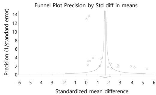
Supplementary Fig. 4. Funnel plot after removing 3 studies: Cha (2019), Cha (2020), and Kim (2010).
