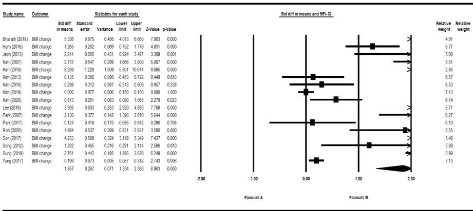
Supplementary Fig. 1. Forest plot after removing two studies: Cha (2019) and Cha (2020).
